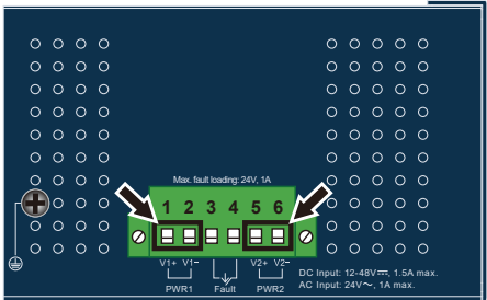
Figure 3-1: IGS-4215-16T2S Inlet Power Socket
